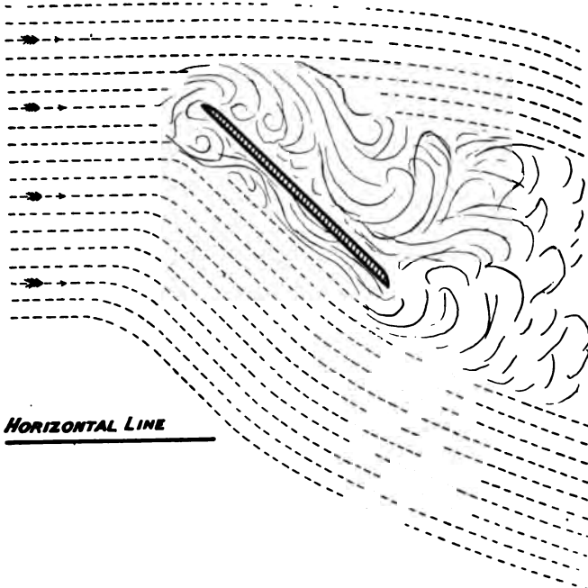
Fig. 64.—Shows a flat aeroplane placed at an angle of 45^\circ , an angle which will never be used in practical flight, but at this angle the momentum of the approaching air and the energy necessary to give it an acceleration sufficiently great to make it follow the back of the aeroplane are equal, and at this point, the wind may either follow the surface or not. Sometimes it does and sometimes it does not. See experiments with screws.
